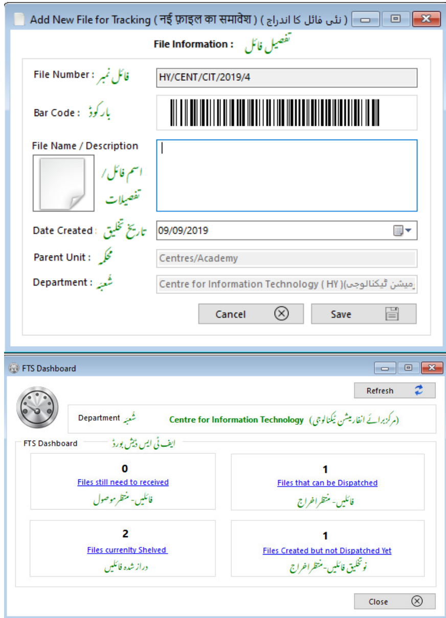
iUMS 2.0 interface for Adding Files and viewing Files Dashboard
